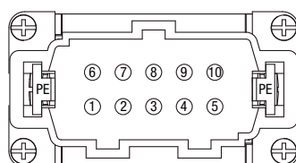
PIN assignment MIG16
