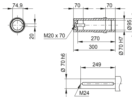
KS09 - Output shaft KB09 - Output shaft on both sides
