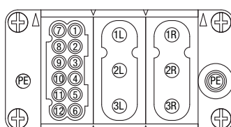
PIN assignment MIG40
