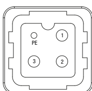
PIN assignment MIG10-FL
