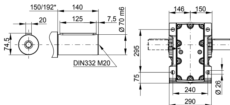
KS09 - Output shaft KB09 - Output shaft on both sides
