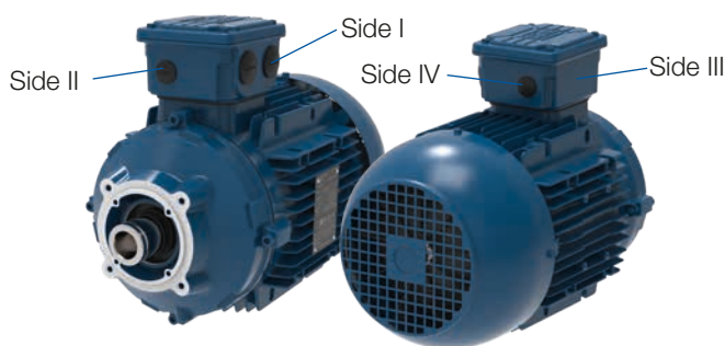
Side designation for cable entries
