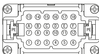
PIN assignment MIG10B
