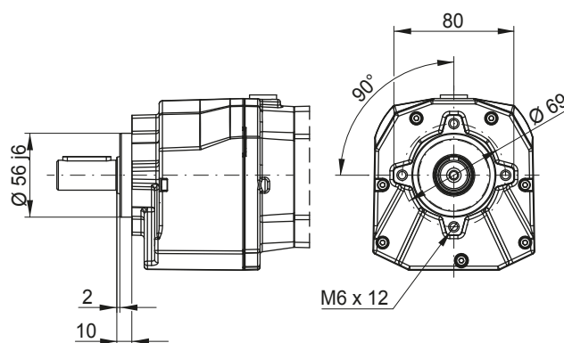
CC00 - B14 flange execution + centring and threaded hole
